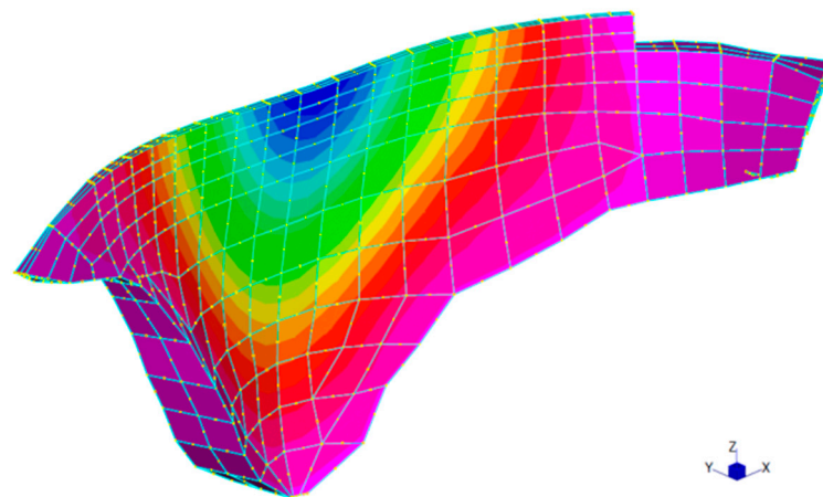
Figure 15. Static loading radial displacement (DY).
