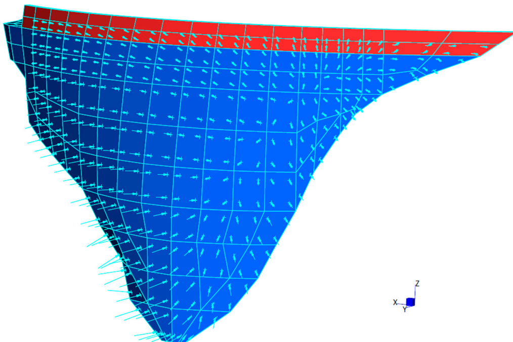
Figure 6. Hydrostatic pressure on upstream wall.
