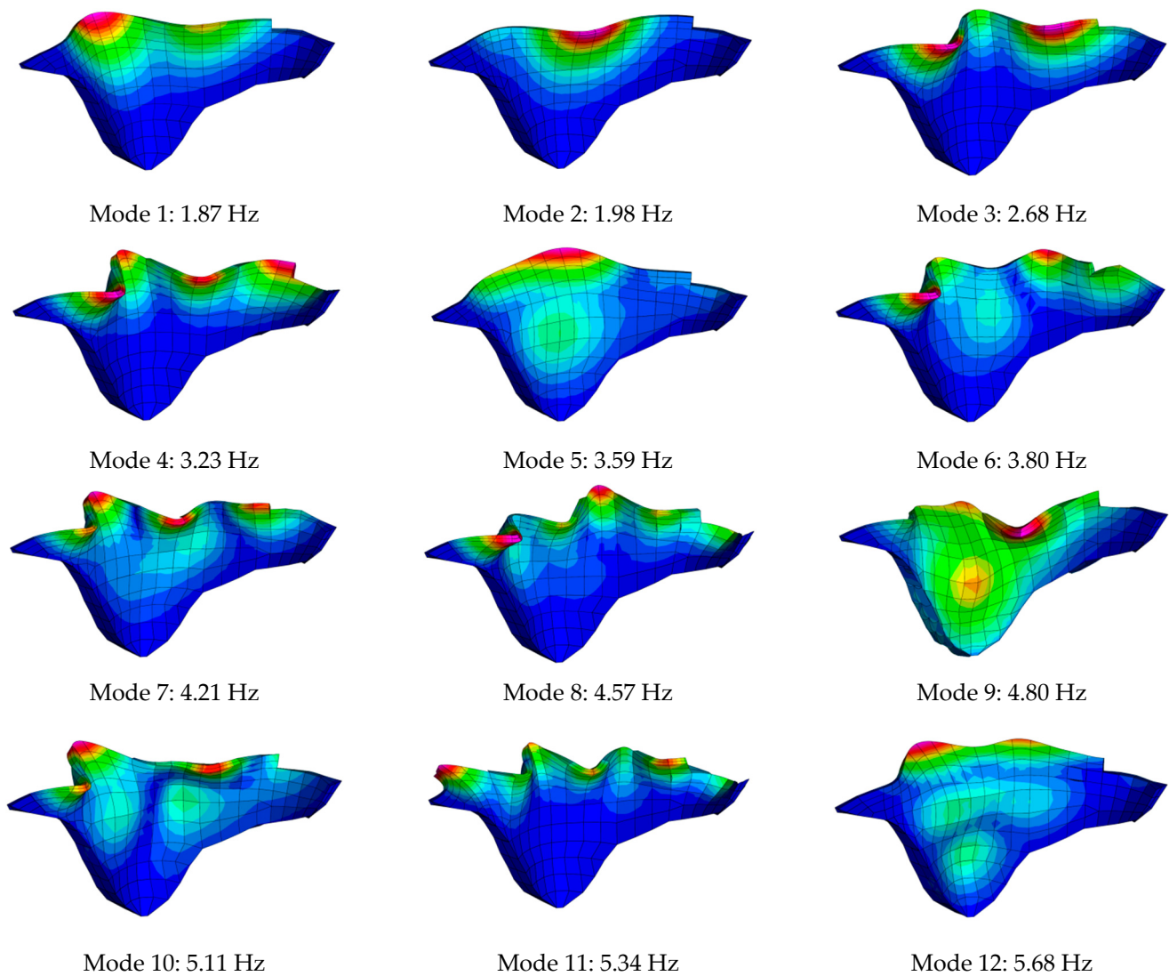
Figure 17. Mode Shapes.
