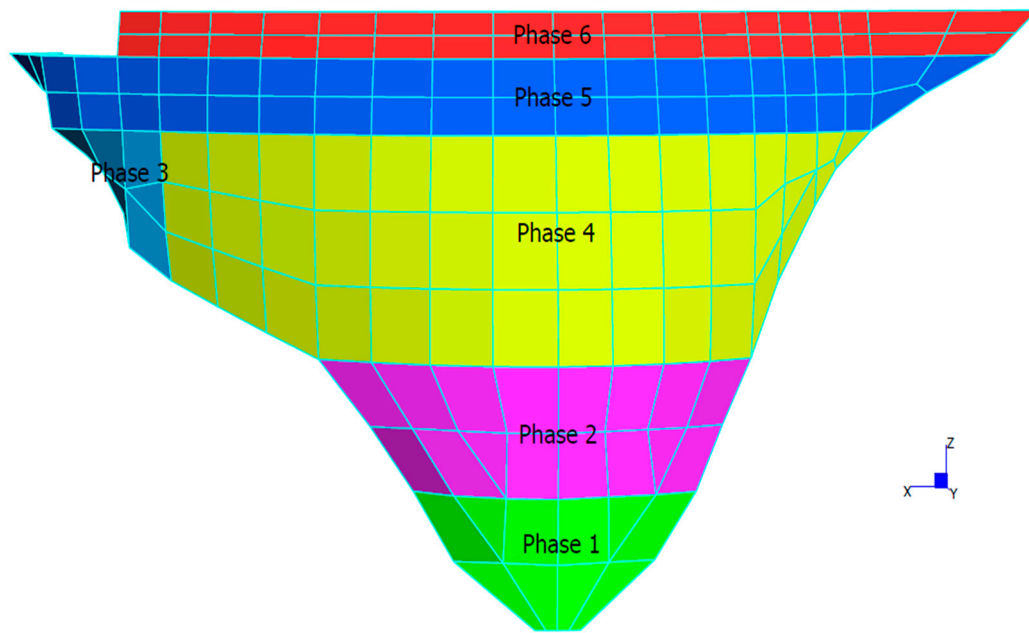
Figure 5. Luzzone dam construction phases.
